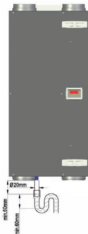
WHR - Links
